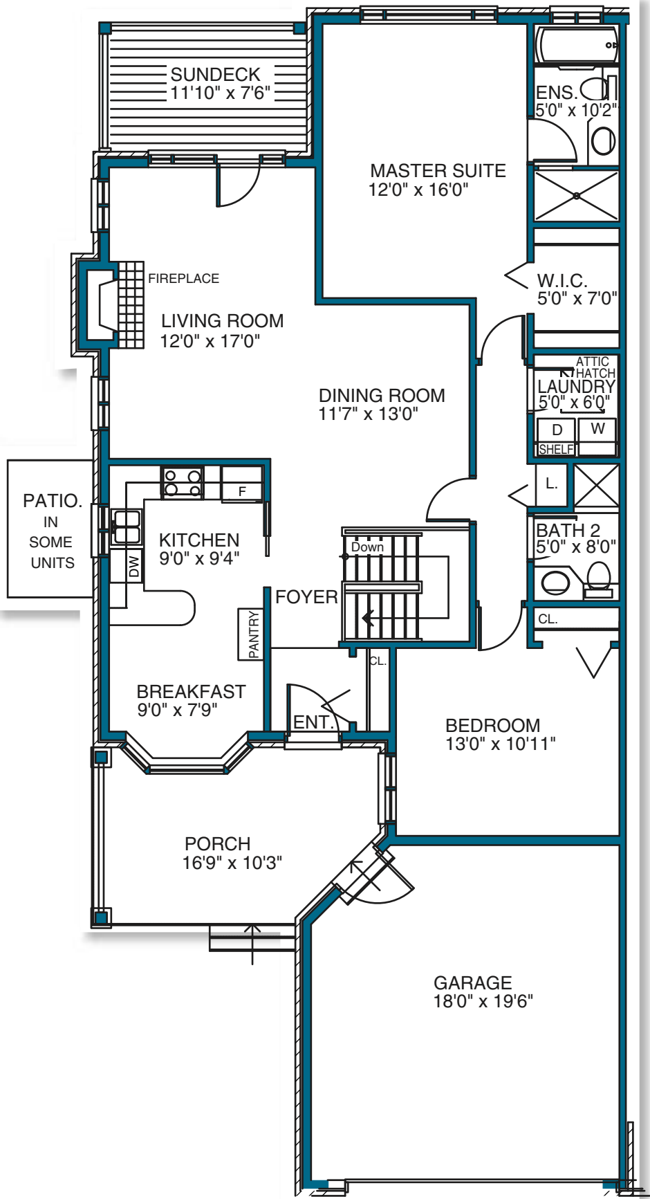
RIVERGLEN MAIN LEVEL PLAN
